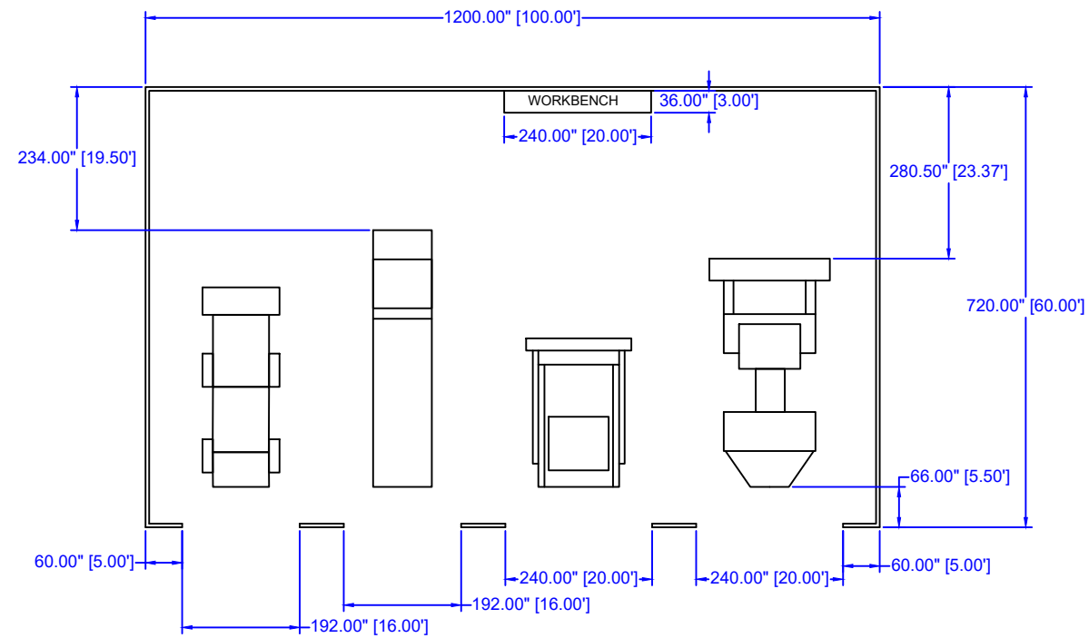
OPTION B LENGTH: 100' WIDTH: 60' Height: 20' DOORS: X2 16' DOORS: X2
