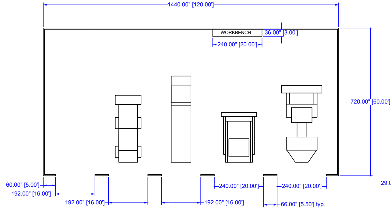
OPTION A LENGTH: 120' WIDTH: 60' Height: 20' DOORS: X2 16' DOORS: X3
