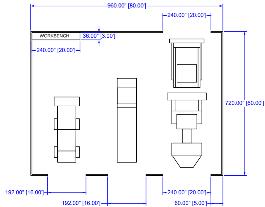
OPTION C LENGTH: 80' WIDTH: 60' Height: 20' DOORS: X2 16' DOORS: X2
